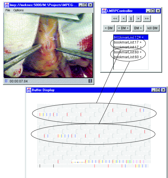
Figure 3: The MPEG-L/MRP demonstrator
