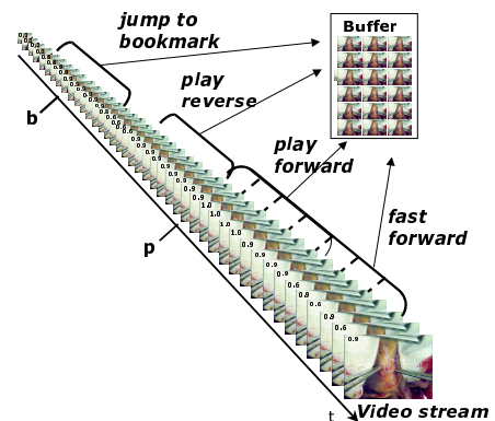
Figure 1: Relevant frames for interactive streaming
