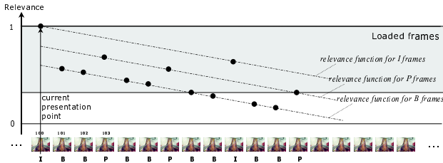
Figure 2: The relevance function for play forward in MPEG-L/MRP
