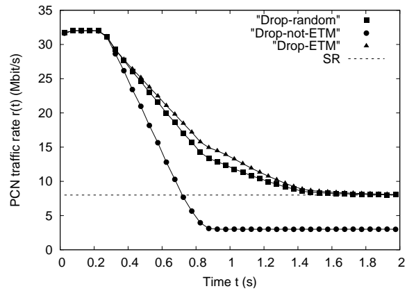
Fig. 6 Impact of packet loss.
