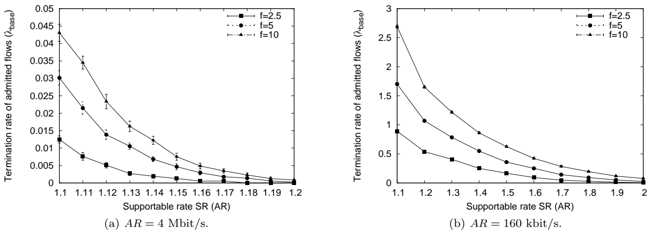
Fig. 10 Simulated termination rates.
