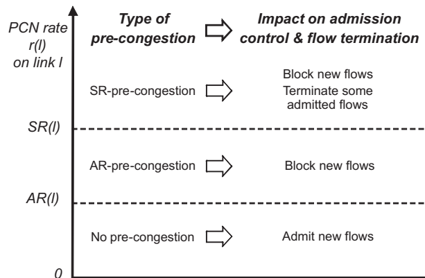
Fig. 1 The admissible and the supportable rate ( AR(l) , SR(l) ) define three pre-congestion states with respect to the PCN traffic rate r(l) on a link.
