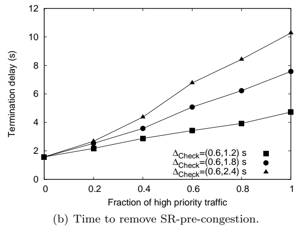
(b) Time to remove SR-pre-congestion.
