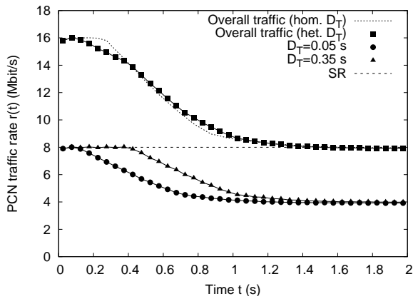
Fig. 5 Impact of heterogeneous termination delay D_T .
