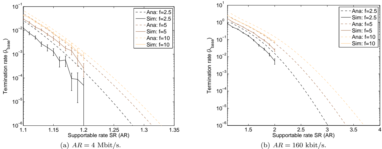
Fig. 12 Simulated and analytically calculated termination rates.
