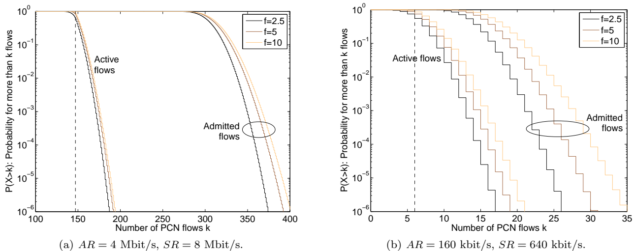
Fig. 13 CCDF for the number of admitted and active PCN flows on bottleneck links with different aggregation levels.
