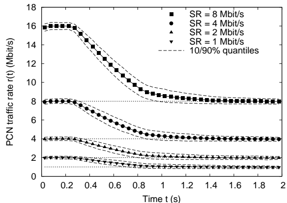
Fig. 4 Impact of traffic aggregation.
