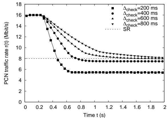
Fig. 2 Impact of the check interval \Delta_{Check} .
