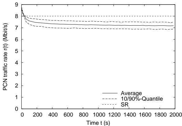
(a) SR = 8 Mbit/s, n_{init} = 1205 on/off flows ( \sim 16 Mbit/s).
