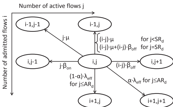
Fig. 11 A snapshot of the state transition diagram visualizes the CTMC.
