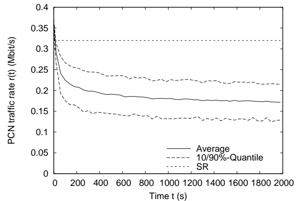
(b) SR = 320 kbit/s, n_{init} = 48 on/off flows ( \sim 640 kbit/s).
