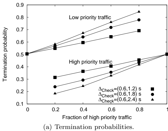
Fig. 7 Impact of flow termination prioritization using different \Delta_{Check} values.
