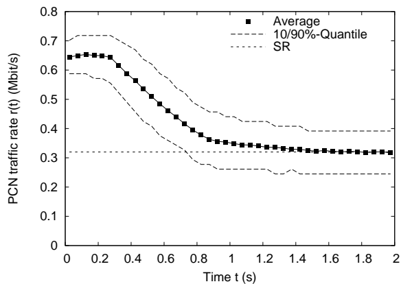
(b) SR = 320 kbit/s, n_{init} = 48 on/off flows ( \sim 640 kbit/s).
