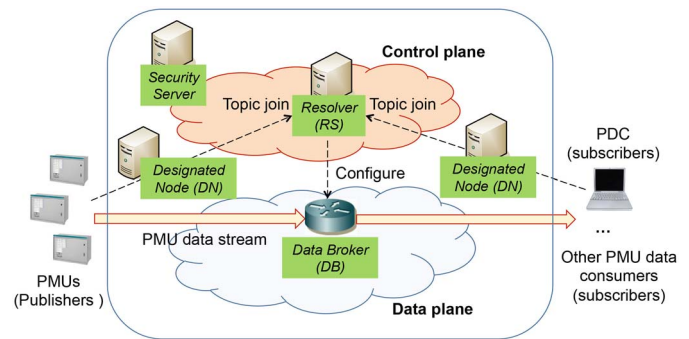
Fig. 2. C-DAX architecture.
