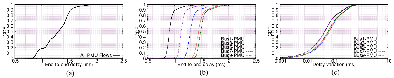
Fig. 7. End-to-end delay and delay variation of PMU flows in the prototype. (Color in online version.) (a) End-to-end delay across all PMU flows. (b) End-to-end delay per PMU flow. (c) Delay variation per PMU flow.
