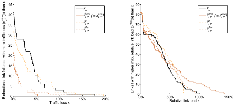
(a) Distribution of traffic loss for all single bidirectional link failures. (b) Distribution of maximum relative load for all unidirectional links.
