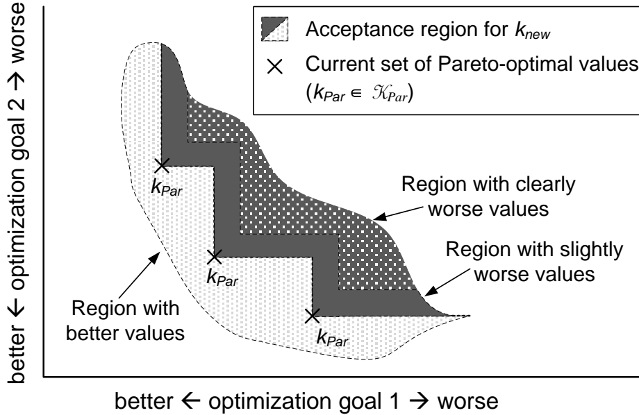
Fig. 8. Threshold Accepting algorithm with two objective functions: acceptance region for a new link cost vector k_{\text{new}} .
