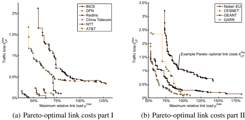
Fig. 9. Percentage of traffic loss \pi_{LP}^{\text{loss}} and maximum link load \rho^{\text{max}} for Pareto-optimal link costs.
