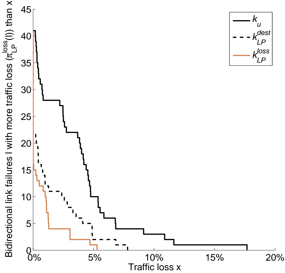
Fig. 6. Distribution of traffic loss for all single bidirectional link failures in the Nobel network when general LFAs are used.
