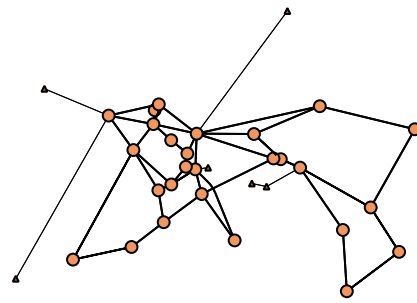
(b) BICS Network: 27 core nodes, 84 uni-direct. links.
